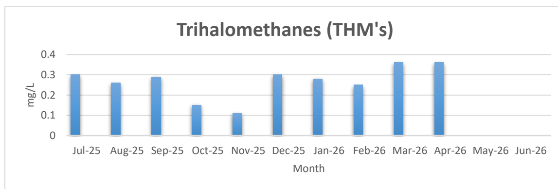
Figure 1: Trihalomethane (THM) values over the recent months (mg/L)
